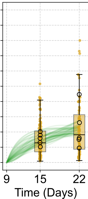
Neurons
